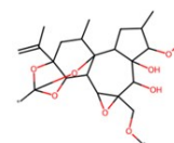
Acyl Structure R1
